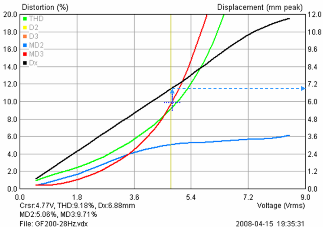
Figure 7. Measurement results for a woofer (black = displacement Dx)
