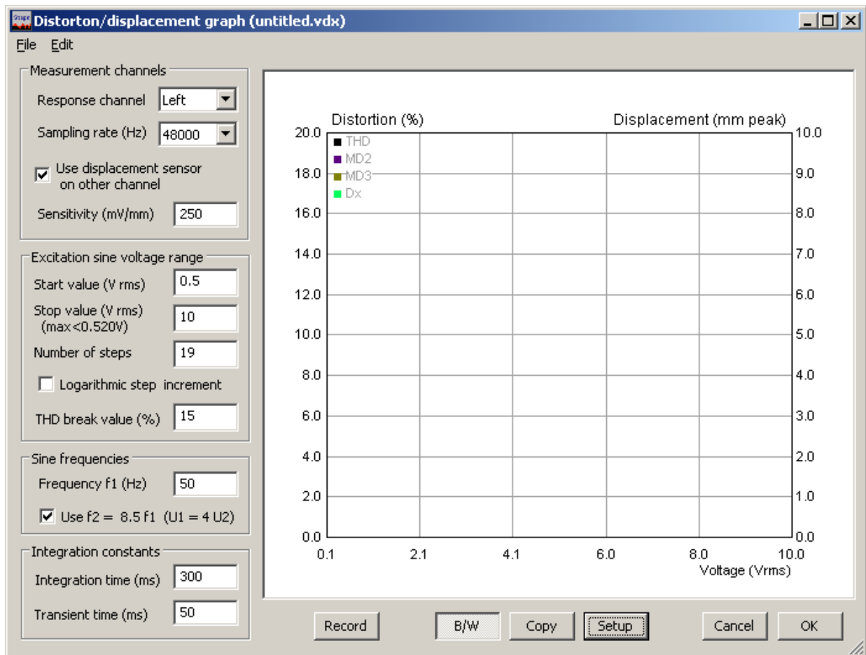
Figure 5. Distortion / Displacement Graph
