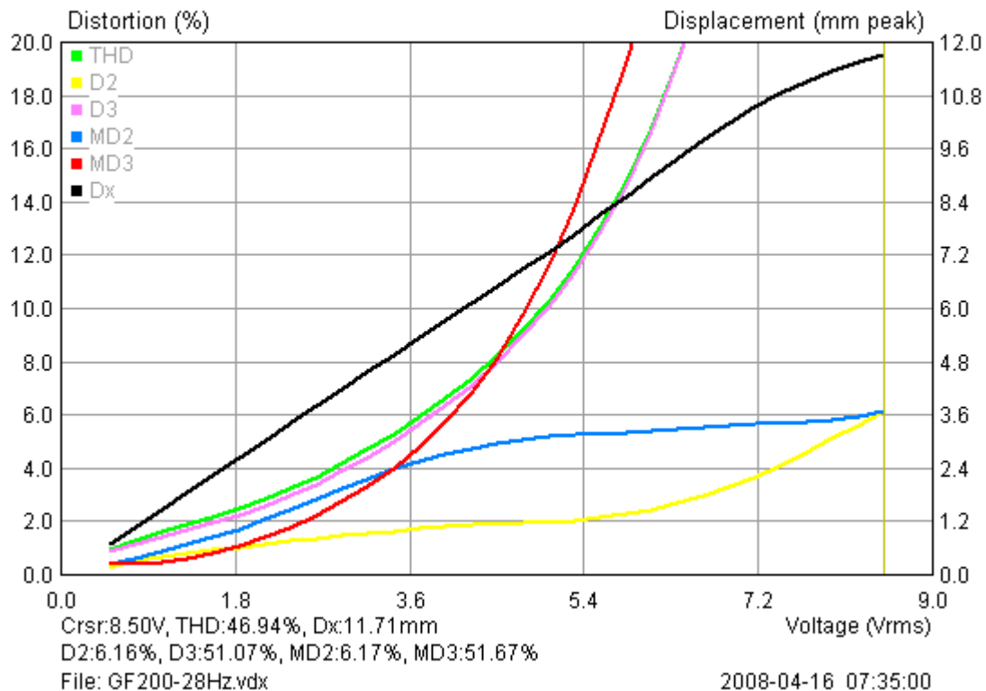
Figure 8. Measurement results with all distortions shown
