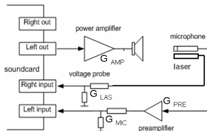
Figure 2. Measurement Setup
