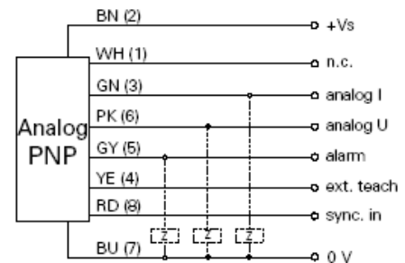
Figure 1. Specification of the Laser Sensor OADM 20I6441/S14F, Baumer [05]
